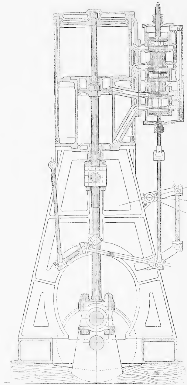
STEEPLE COMPOUND ENGINE WITH CANFIELD'S VALVE.
